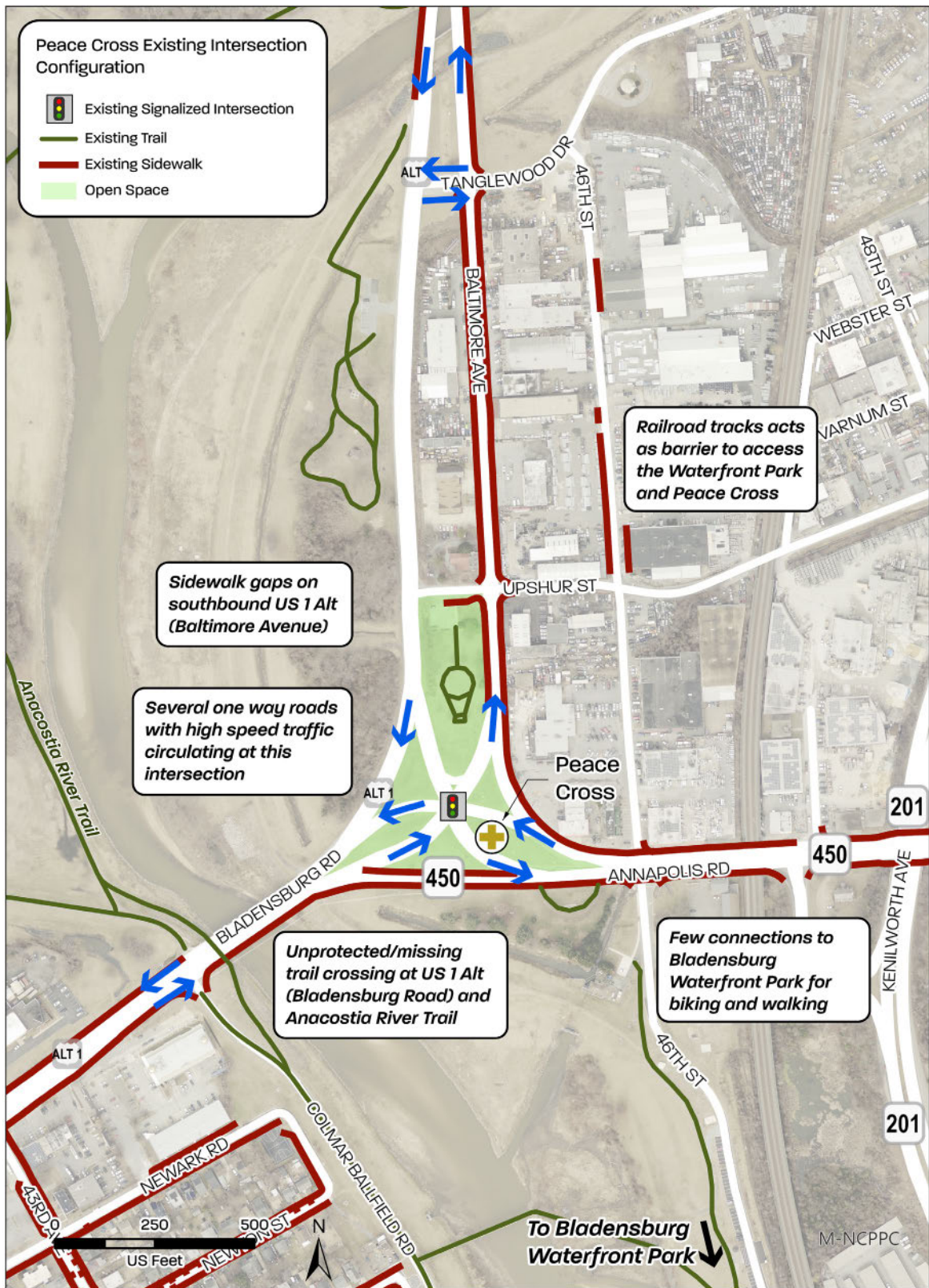
Map 41. Peace Cross Existing Intersection Configuration 207
