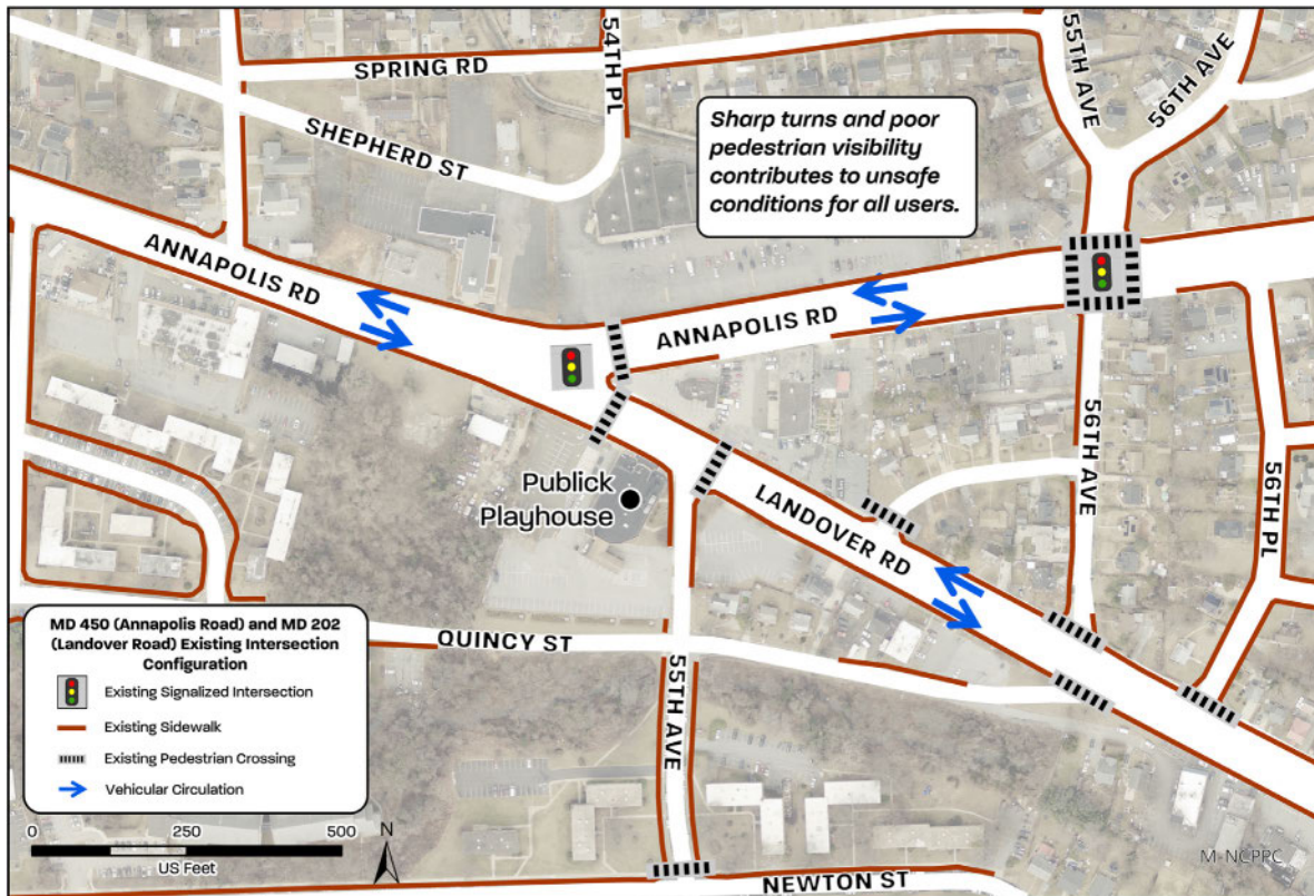
Map 43. MD 450 (Annapolis Road) and MD 202 (Landover Road) Existing Intersection Configuration
