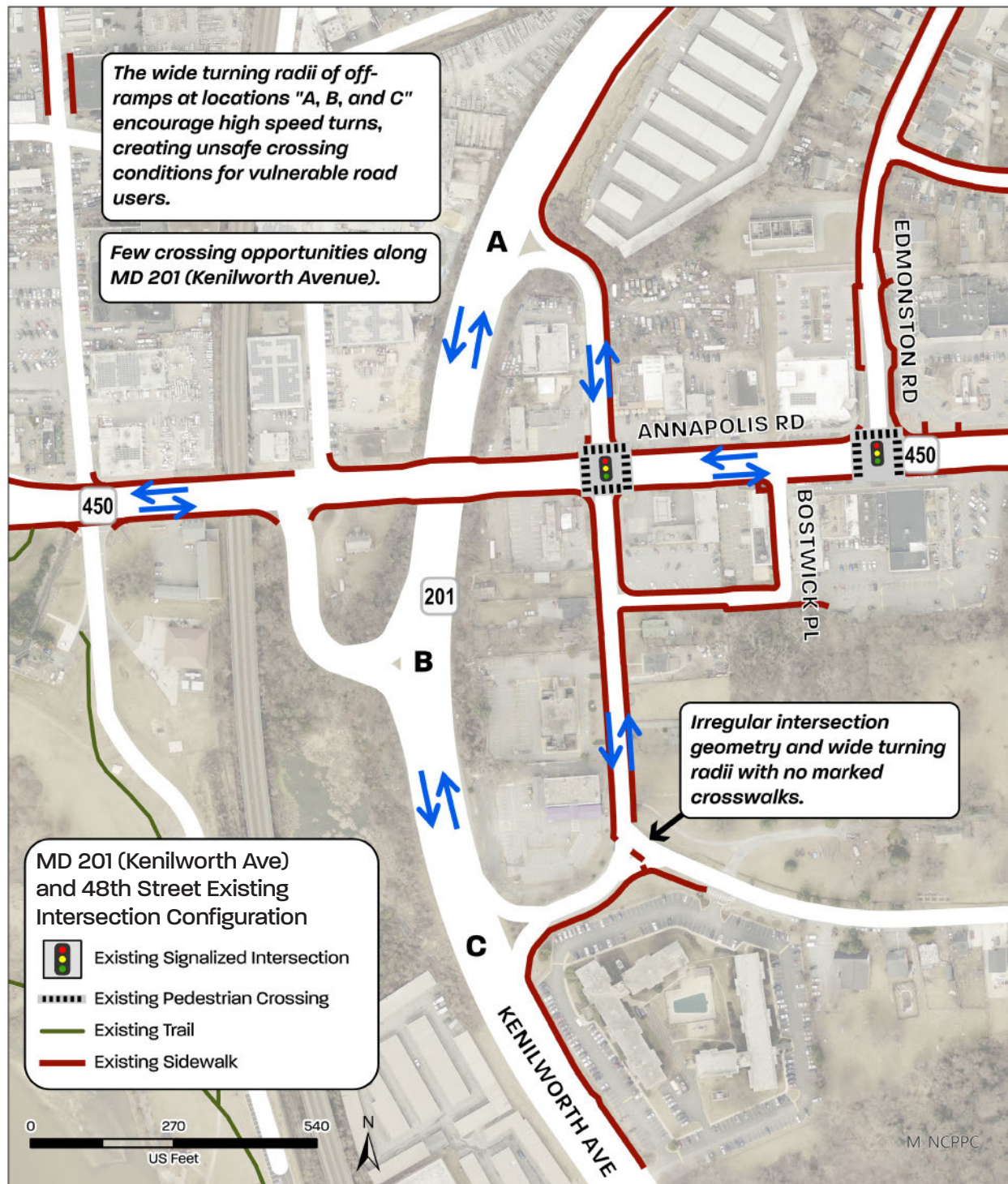
Map 45. MD 201 (Kenilworth Avenue) and 48th Street Existing Intersection Configuration
