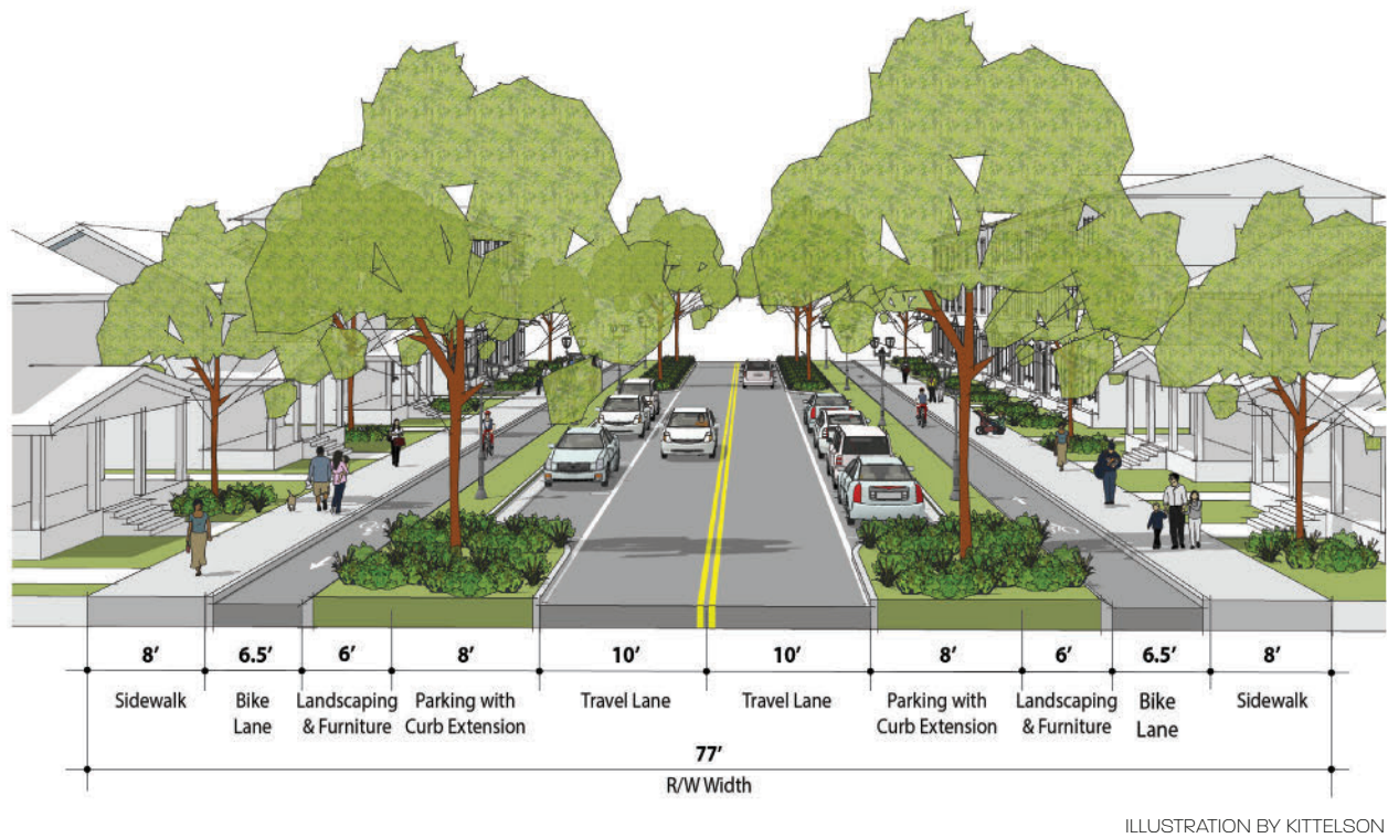
Figure 33. Neighborhood Connector with Separated Bike Lanes 207,288
