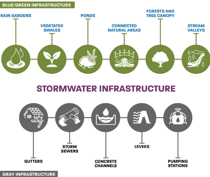
Figure 44. Blue-Green versus Gray Stormwater Infrastructure 98
